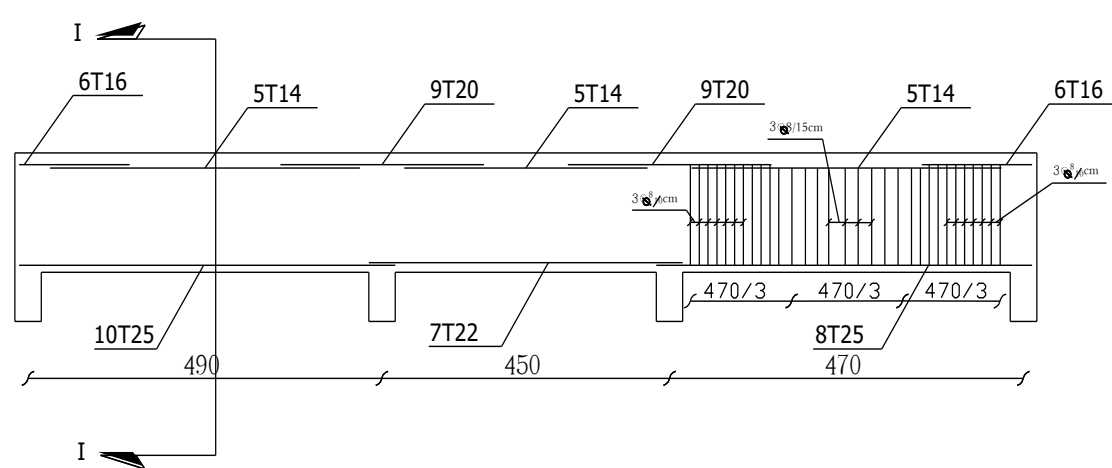
Section in Beam 1 Scale 1/20
