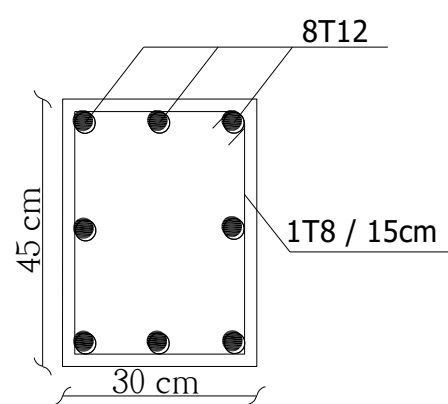
Section in column 1 Scale 1/20
