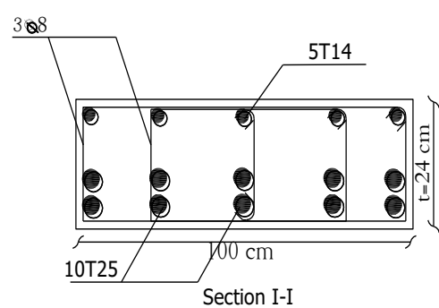
Section in Beam 1 Scale 1/20
