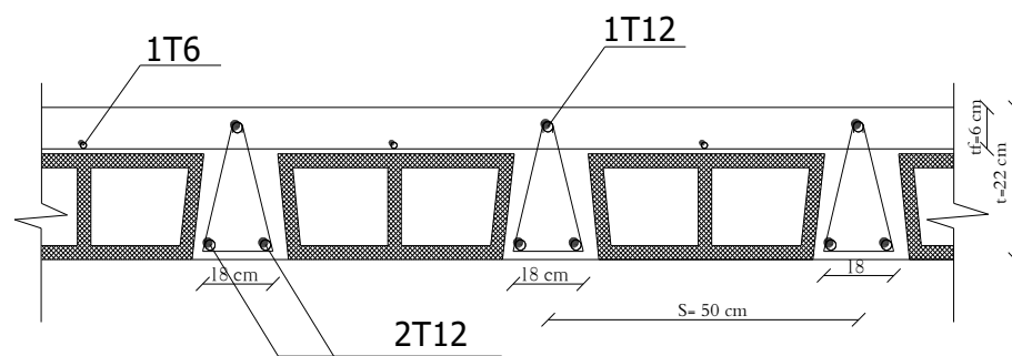
Section in Rib 1 Scale 1/20
